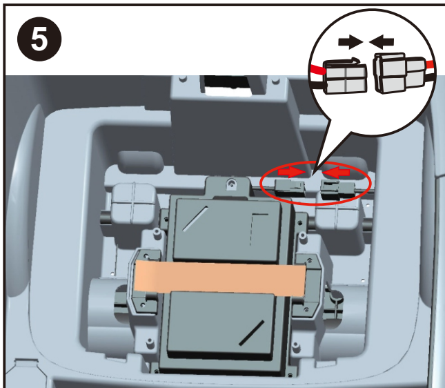
Battery assembly: Plug connectors as the picture.
