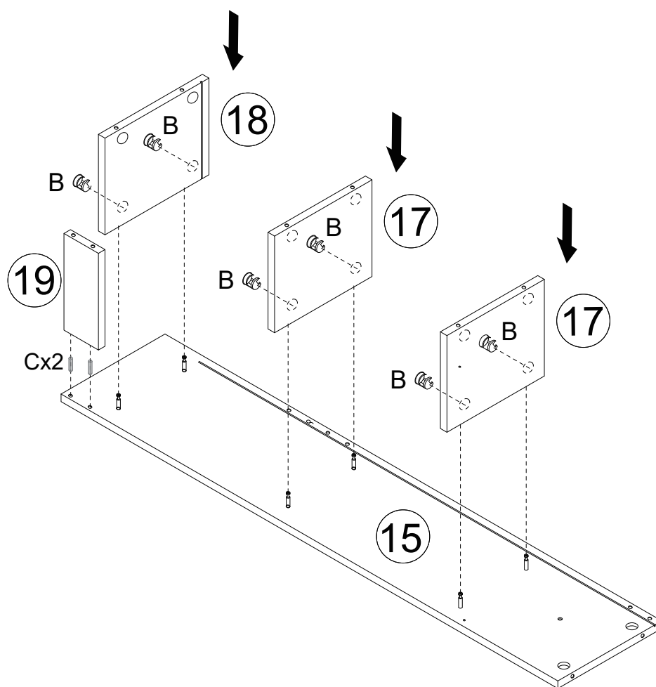
Scheme 2
