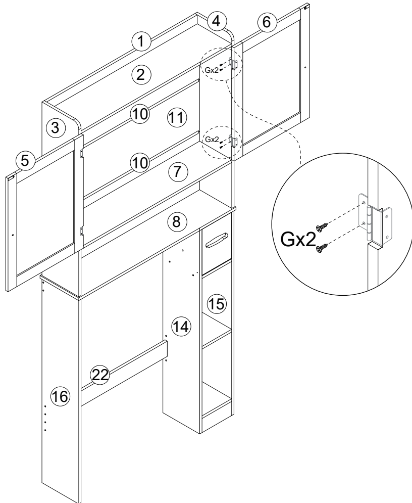
Scheme 2
