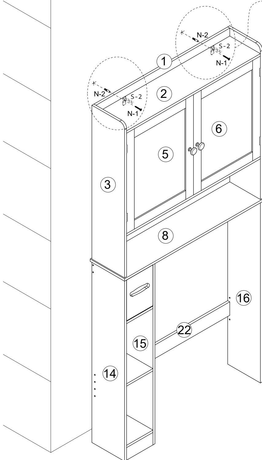
Scheme 1
