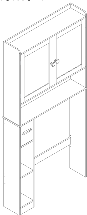
Scheme 1
