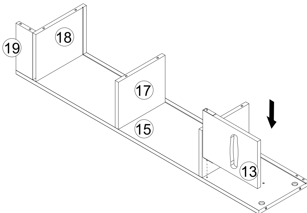
Scheme 2
