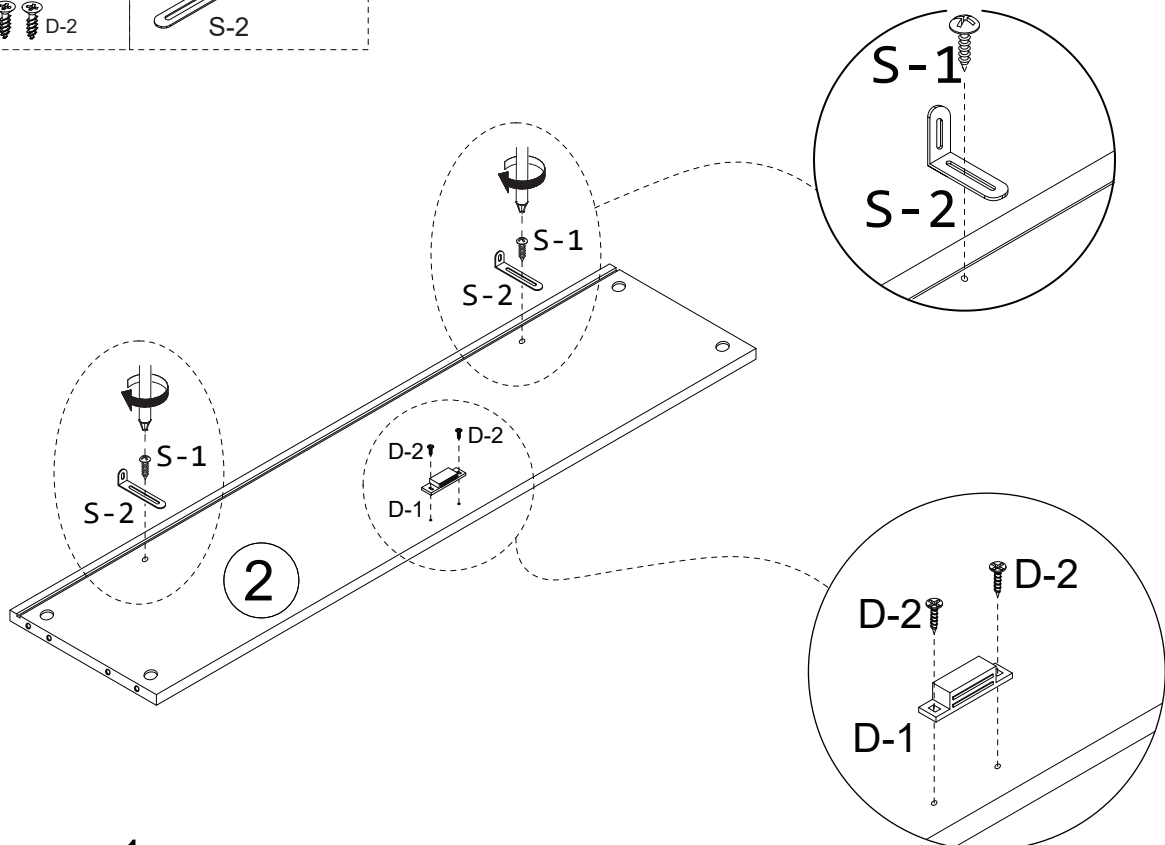
Scheme 1
