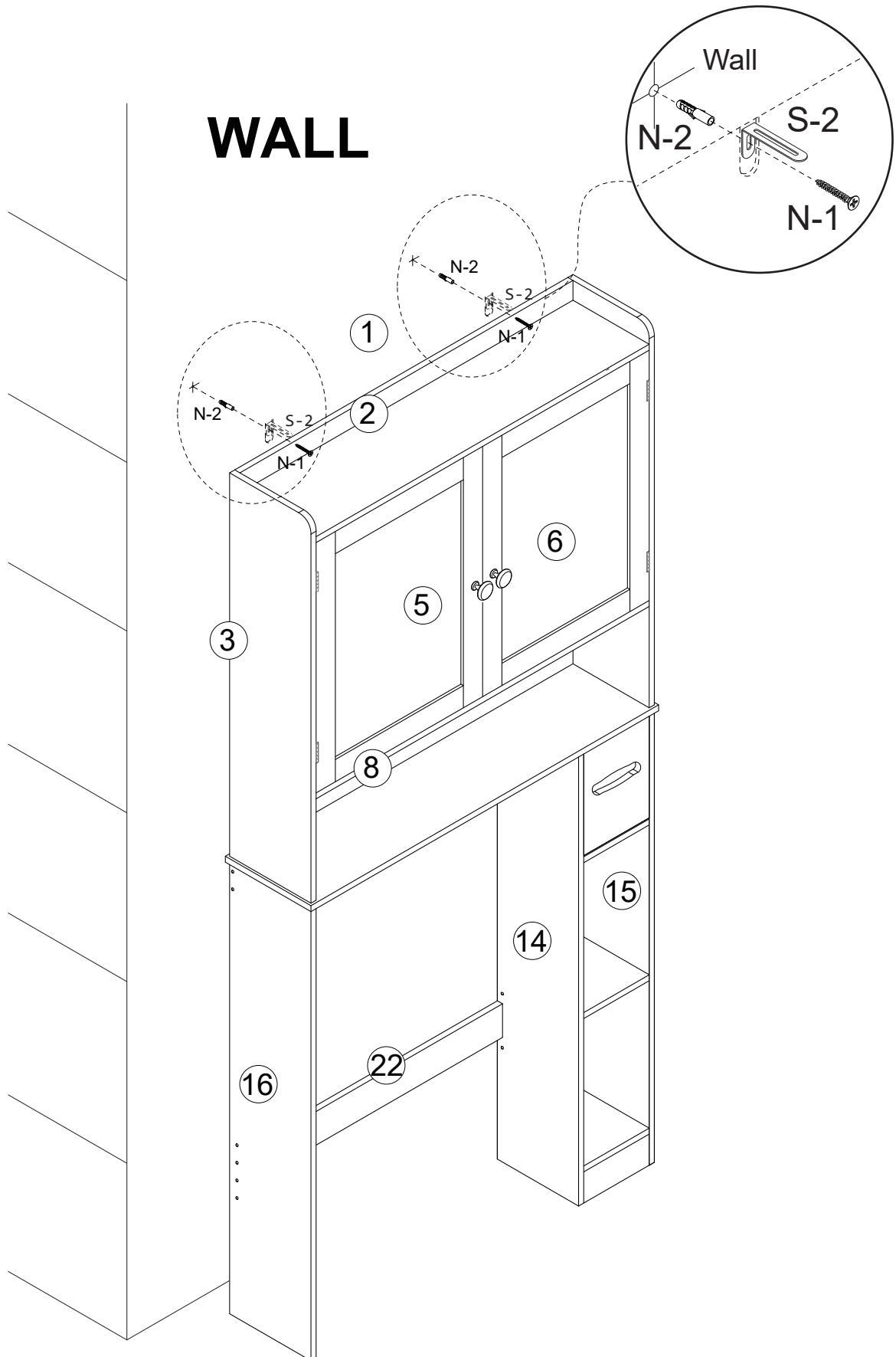
Scheme 2
