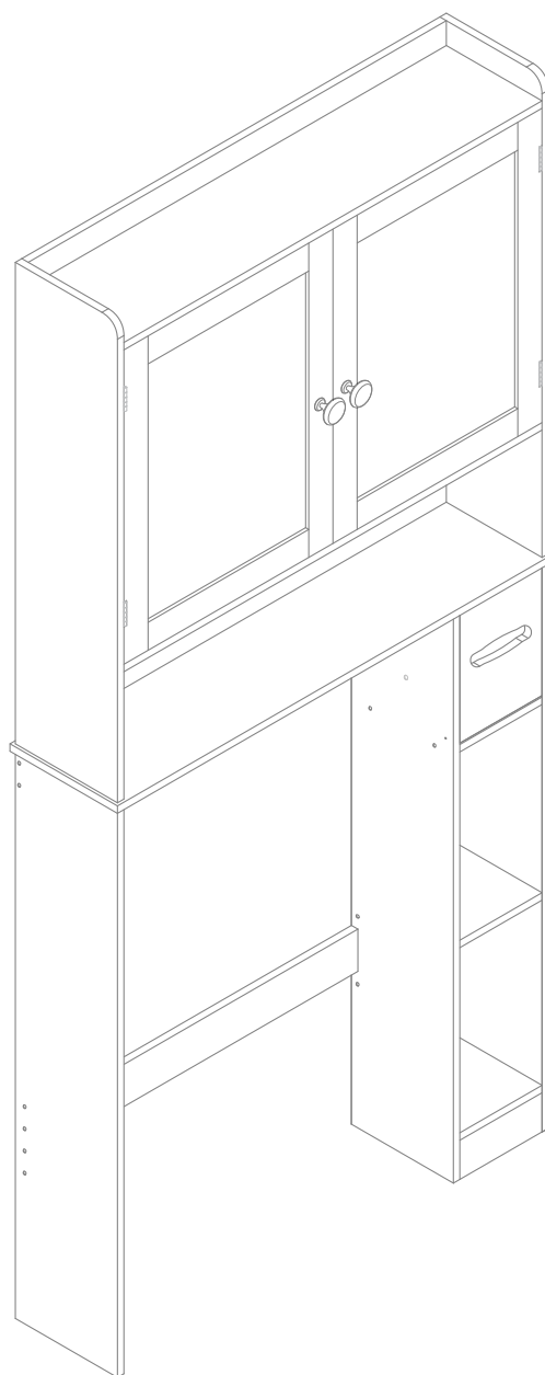
Scheme 2
