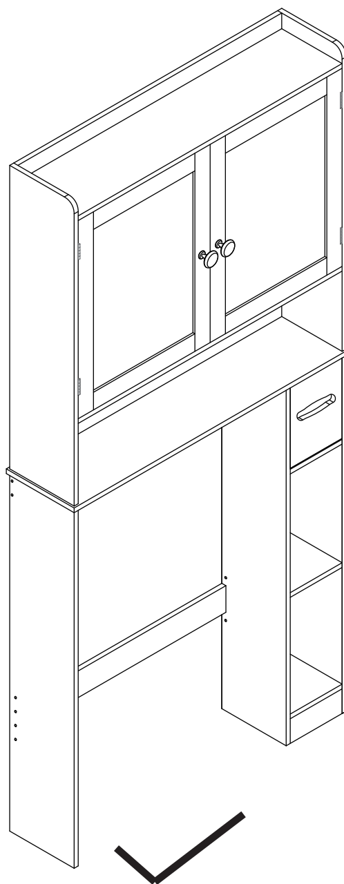
Scheme 2
