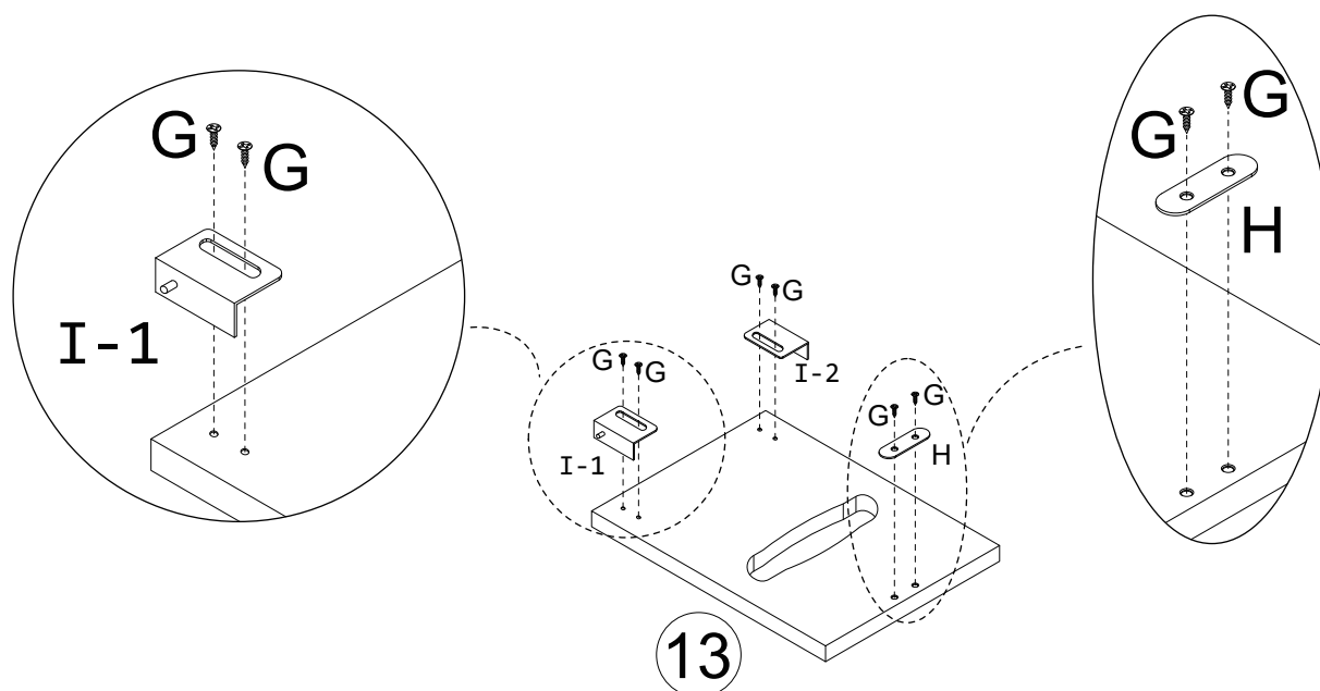
Scheme 2
