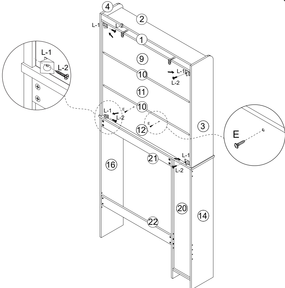
Scheme 1
