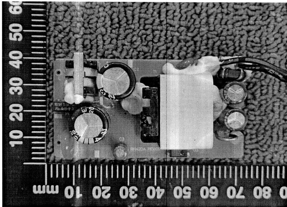
Figure 5. Top PCB view (model: RH-***-****U1)
