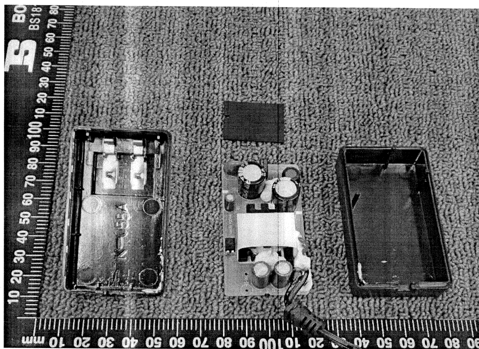
Figure 3. Internal view (model: RH-***-****U1)
