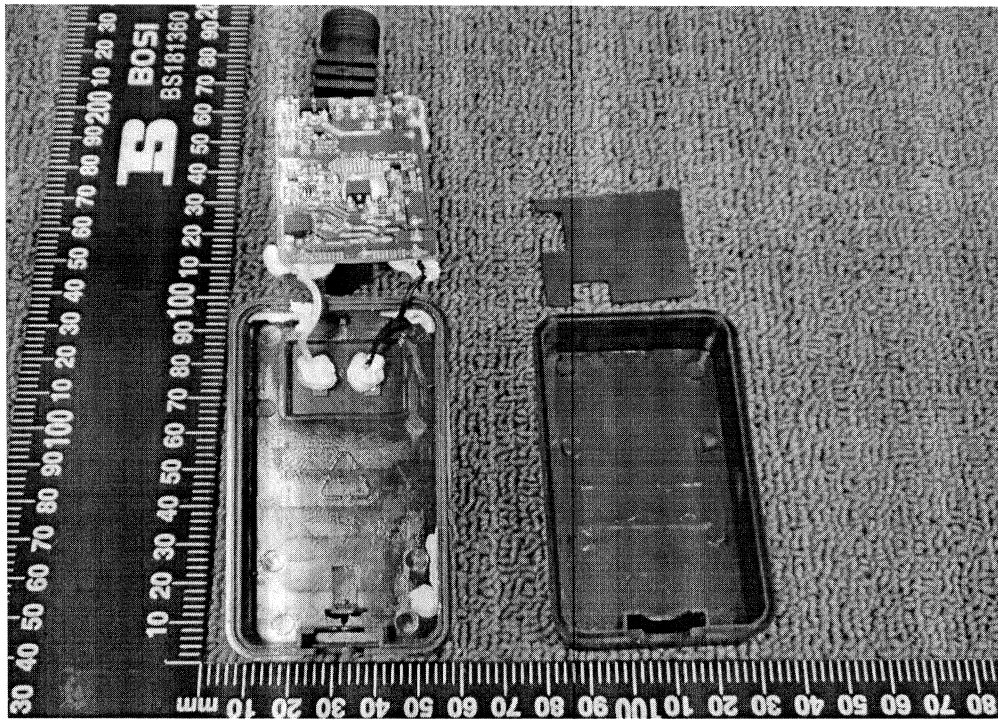
Figure 9. Internal view (model: RH-***-****U4)
