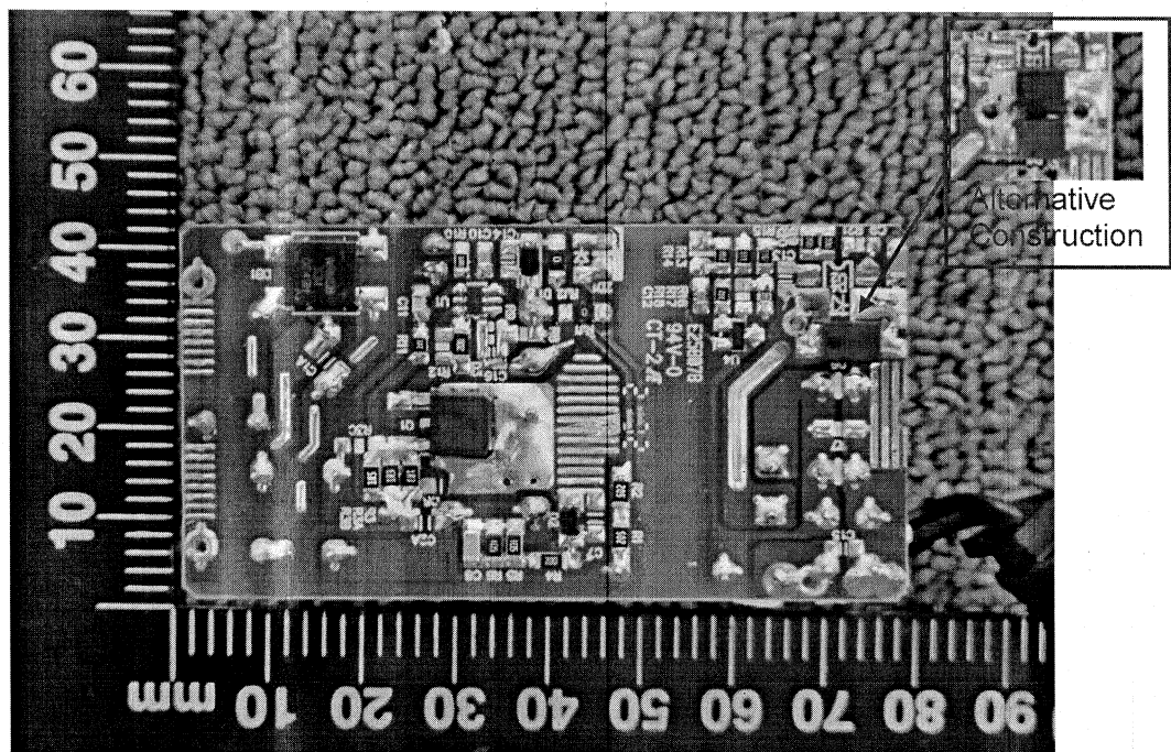
Figure 6. Bottom PCB view (model: RH-***-****U1)
