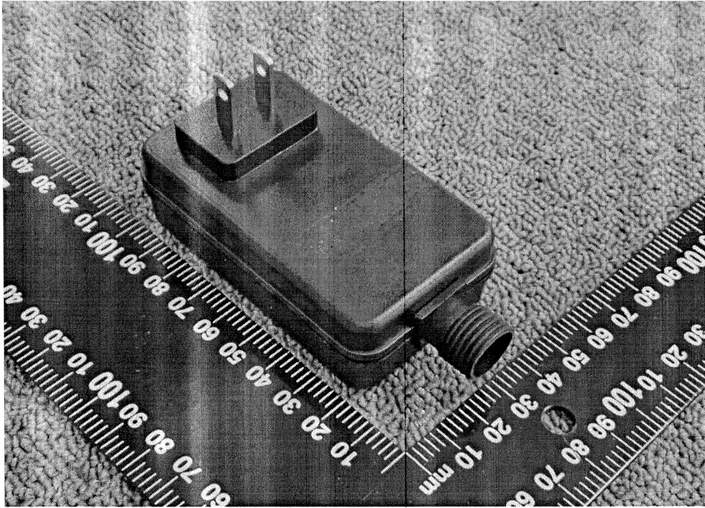
Figure 7. Overall view (model: RH-***-****U4)
