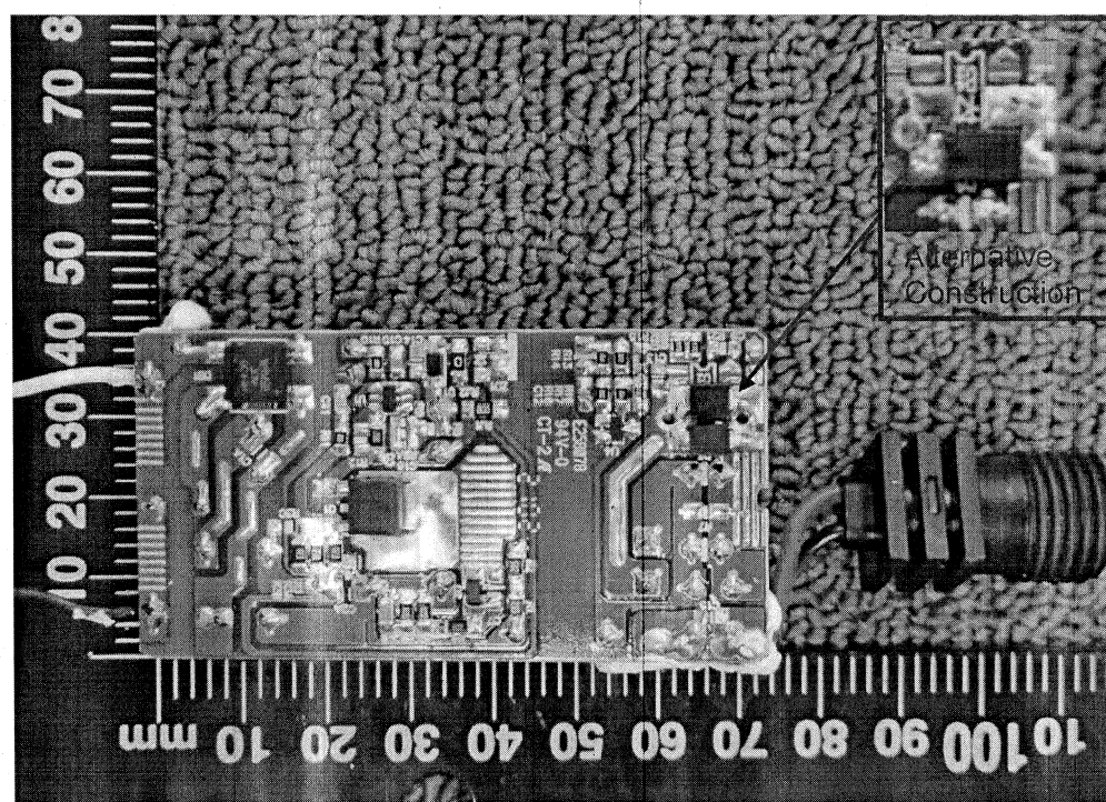
Figure 12. Bottom PCB view (model: RH-***-****U4-1)
