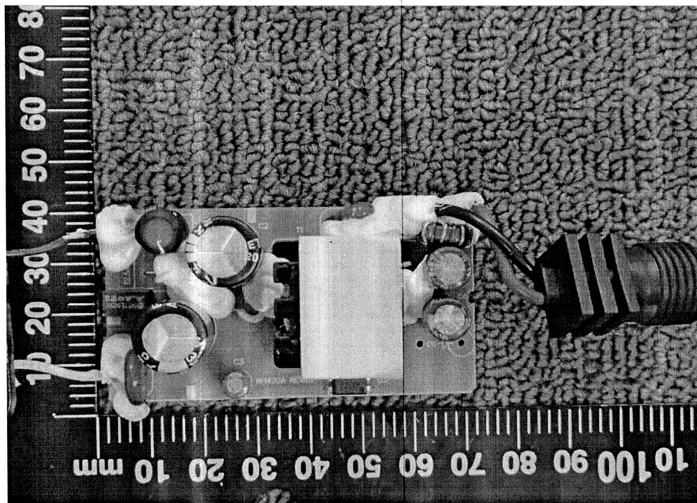
Figure 10. Top PCB view (model: RH-***-****U4)
