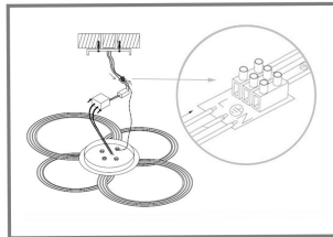
Step 7: Connect the wire through the terminal block.
