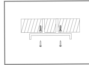
Step 6: Install the hanging bracket by screw on the ceiling
