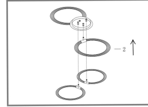
Step 3: Fix 2nd ring's thread pole to the ceiling case by the nut which through the wire
