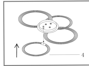
Step 5: Fix 4th ring's thread pole to the ceiling case by the nut which through the wire
