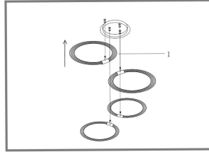
Step 2: Fix 1st ring's thread pole to the ceiling case by the nut which through the wire
