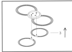
Step 4: Fix 3rd ring's thread pole to the ceiling case by the nut which through the wire
